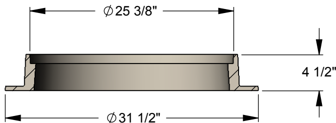
SECTION VIEW
