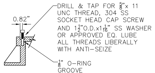
BOLT DETAIL
